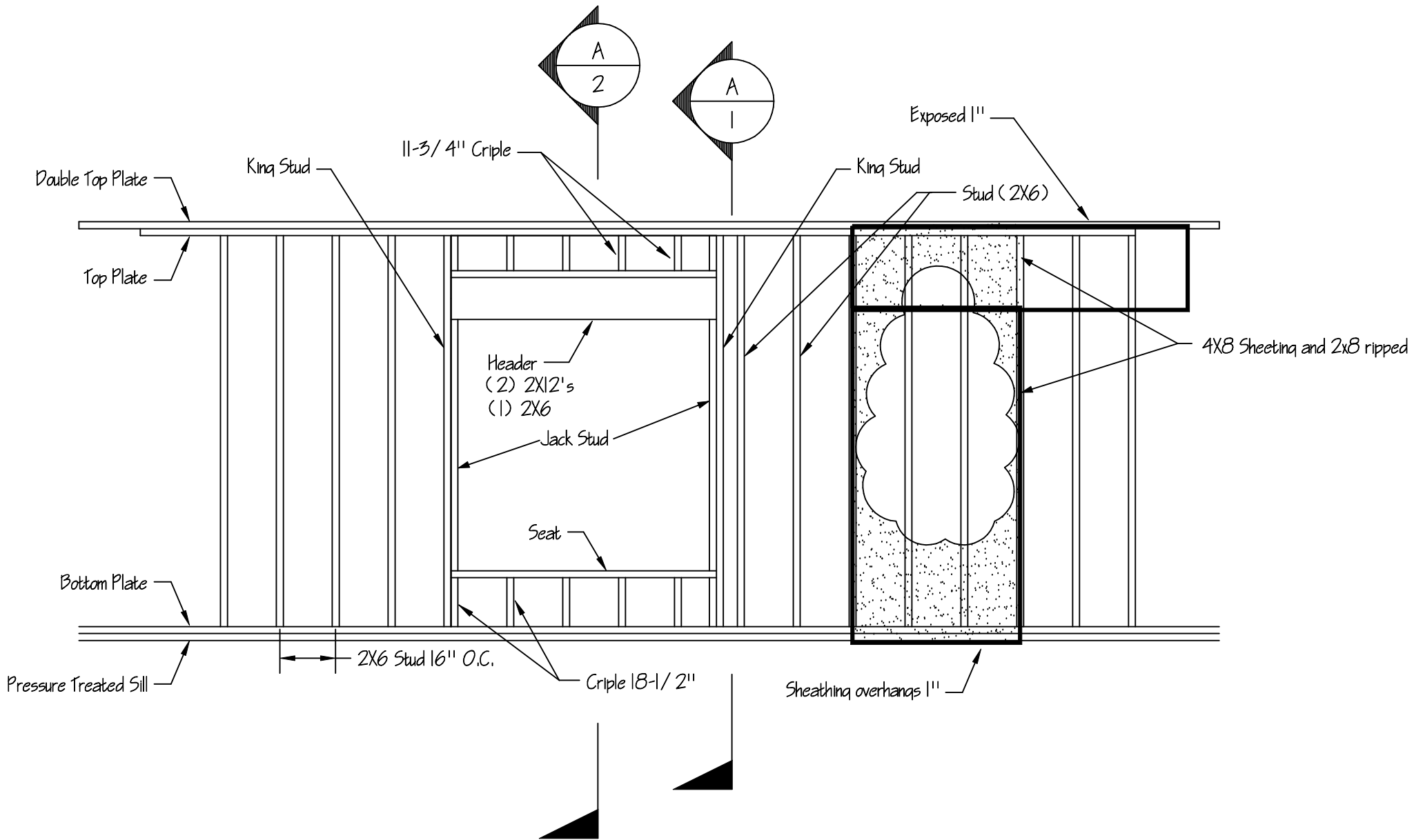
Typical window framing detail
